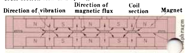
Cross section view of diaphragm
